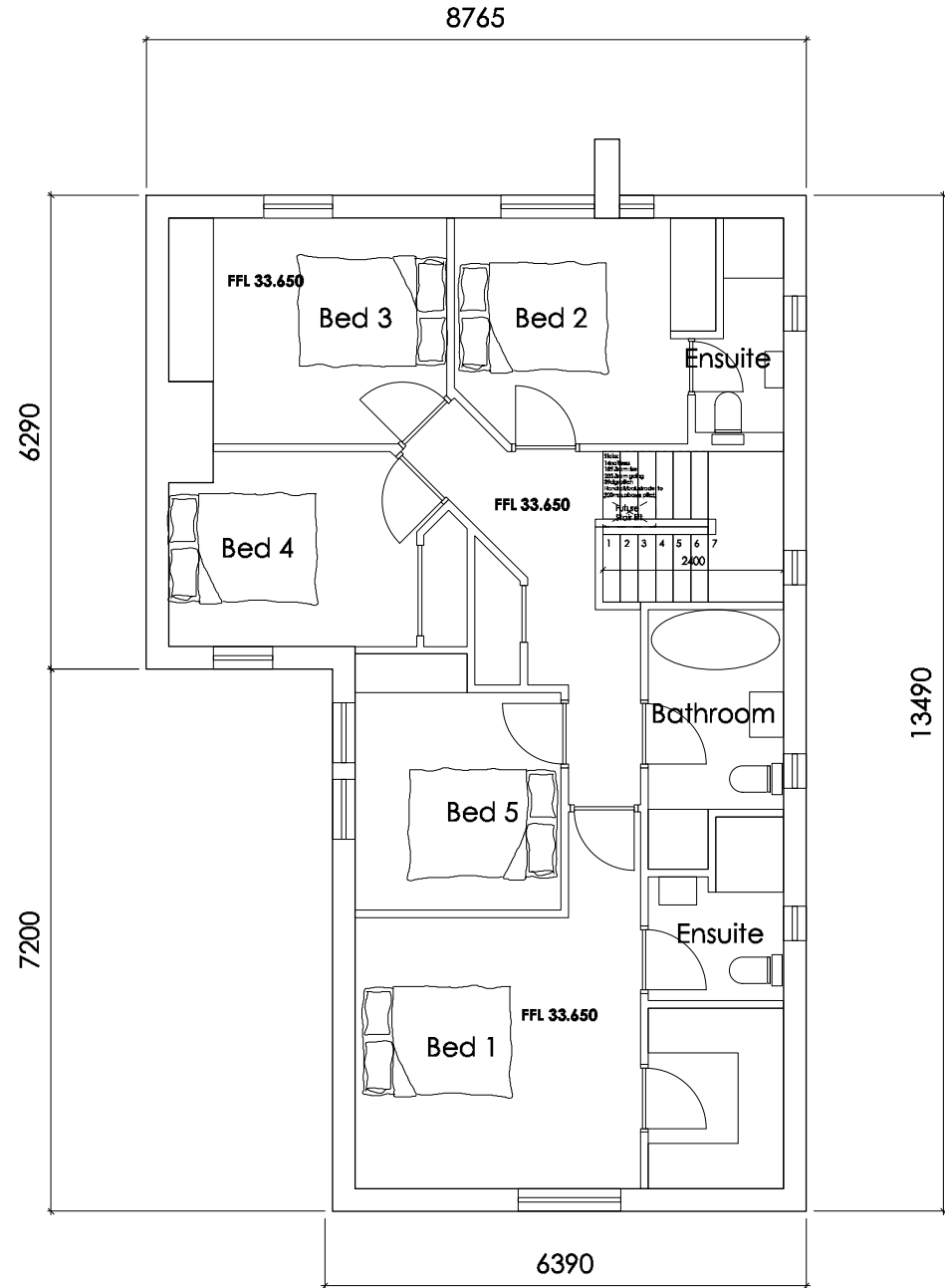
Plot 6 - Proposed 1st floor plan
