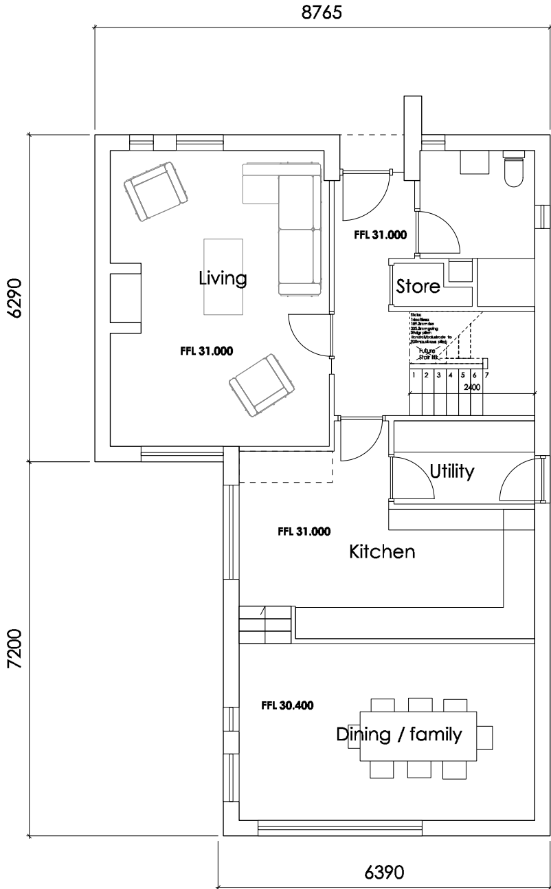
Plot 6 - Proposed ground plan
