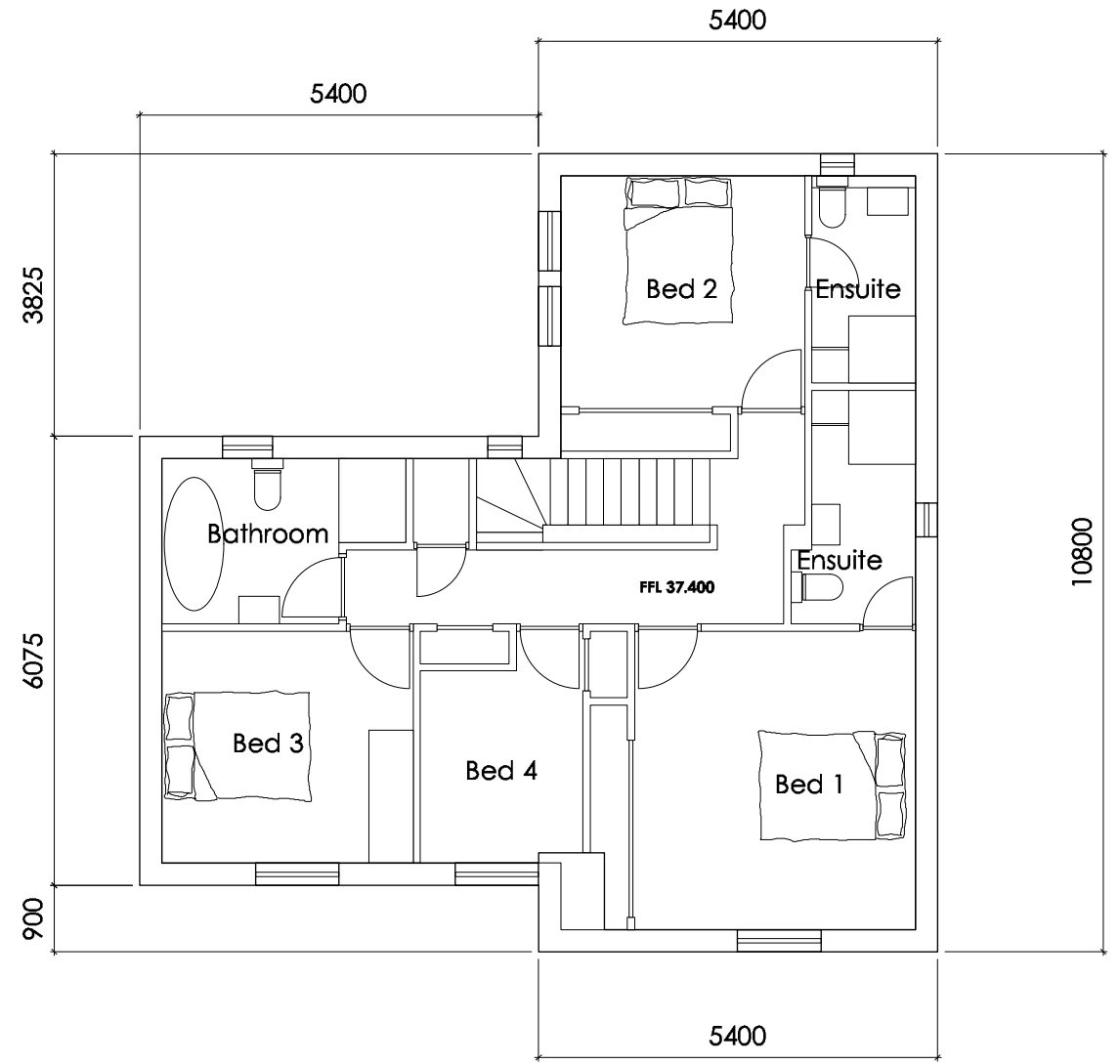
Plot 5-Proposed 1st floor plan
