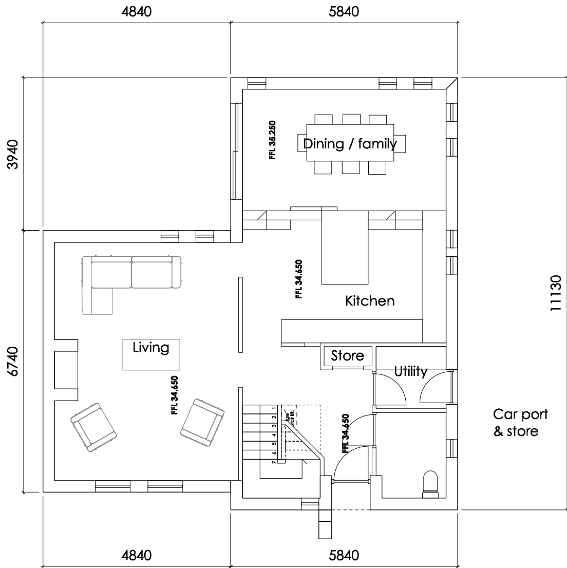
Plot 3 & 4 - Proposed ground plan
