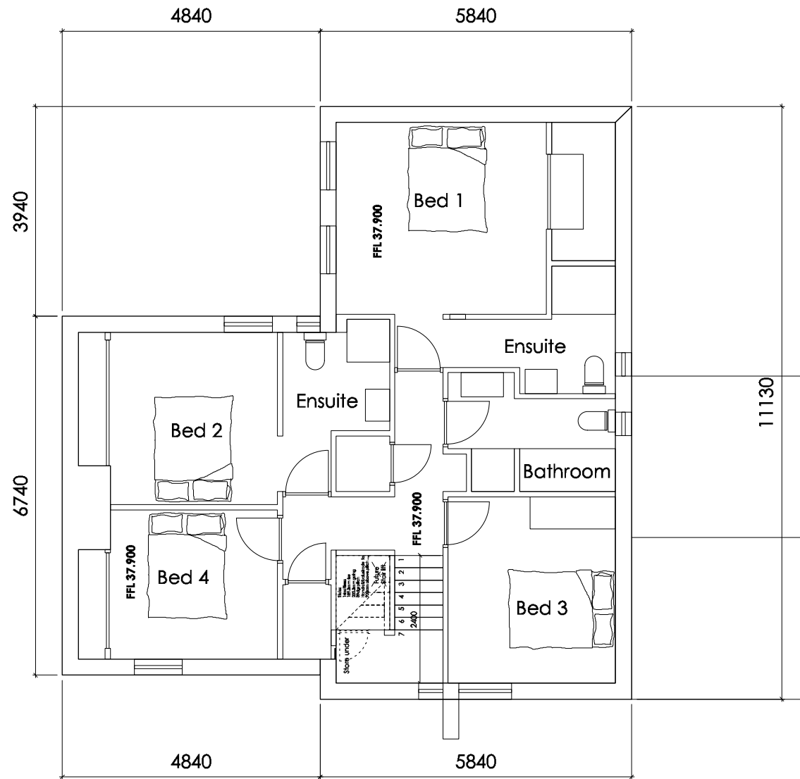
Plot 3 & 4 - Proposed 1st floor plan
