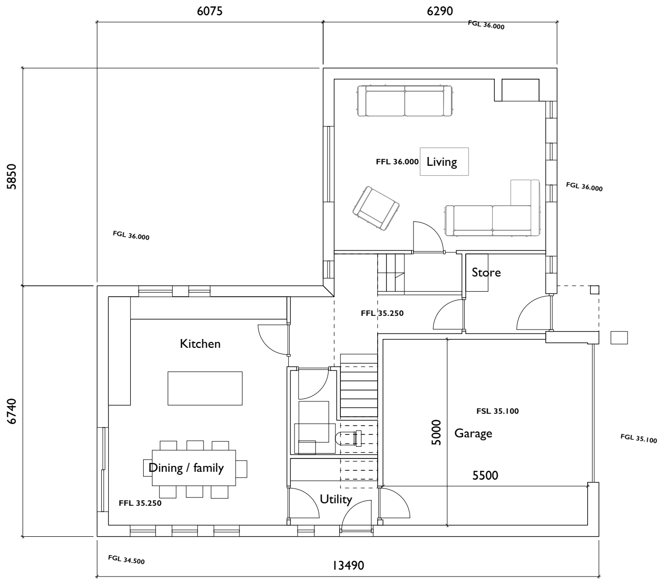
Plot 2-Proposed ground plan
