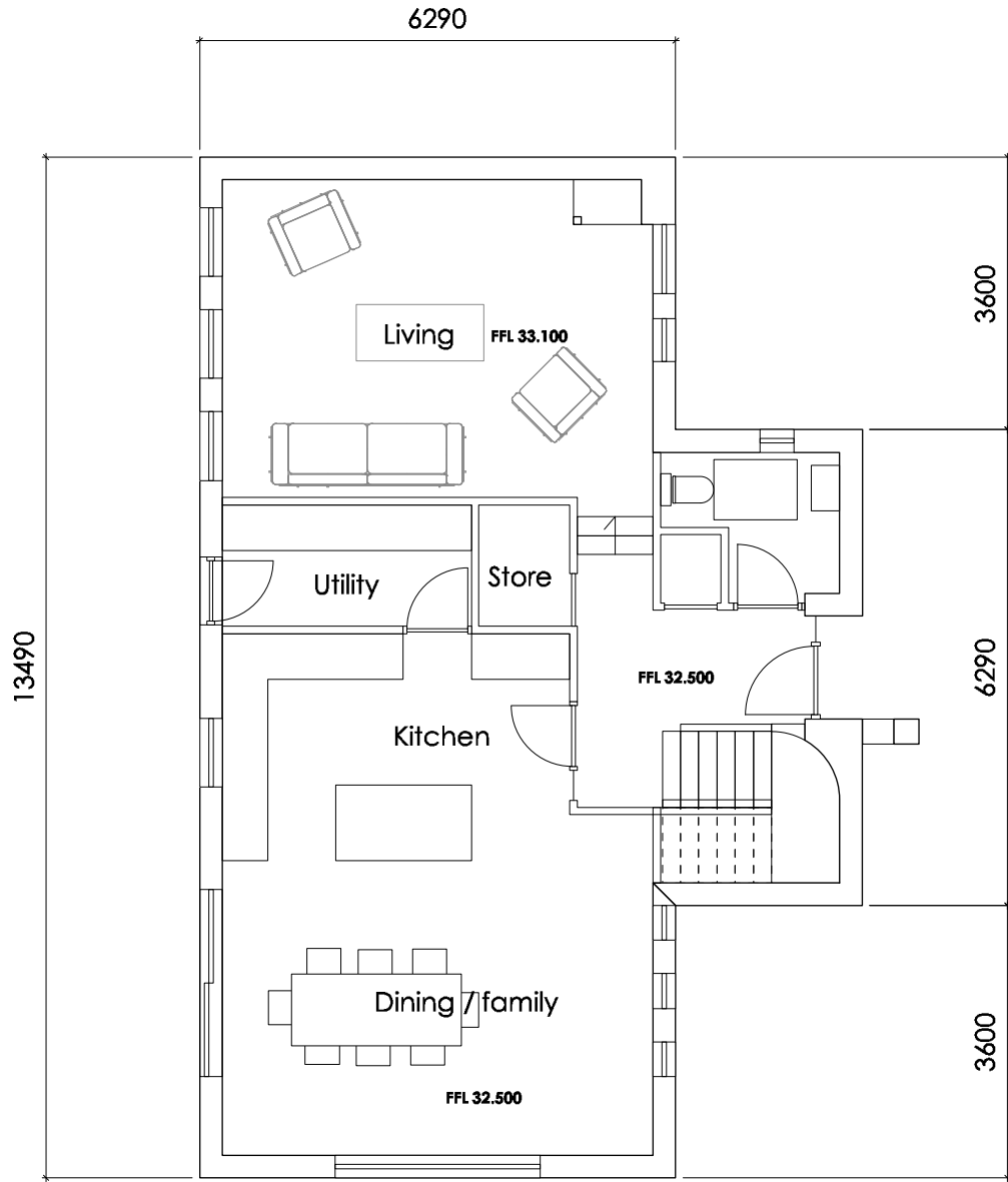
Plot 1 - Proposed ground plan
