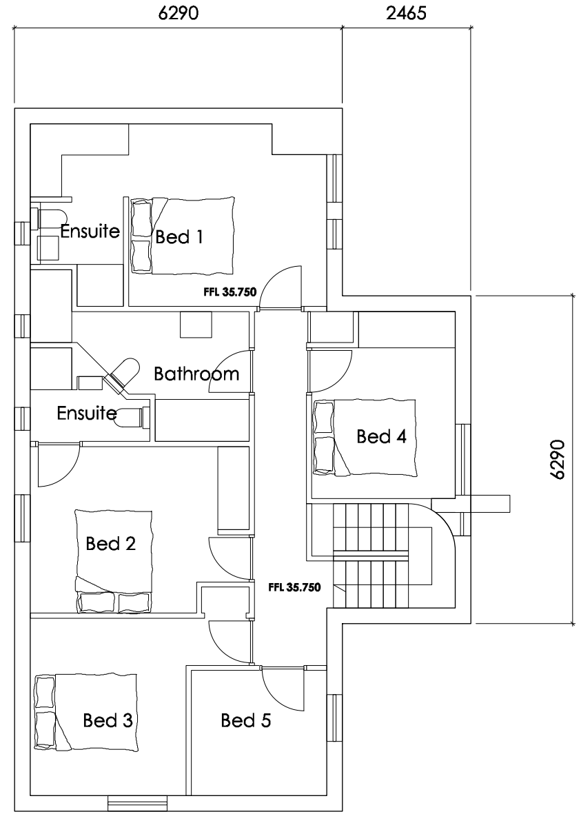
Plot 1 - Proposed 1st floor plan
